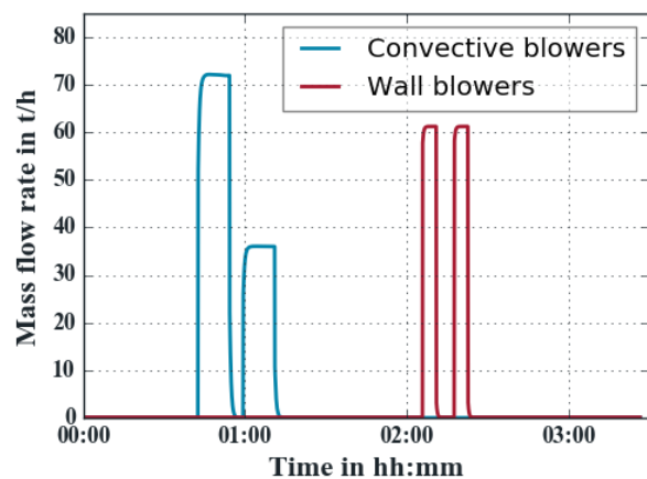
Figure 4. Soot blower injection mass flows
